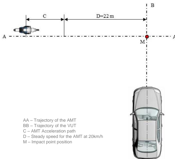
Figure 12: CMCrossing scenario (nearside)
