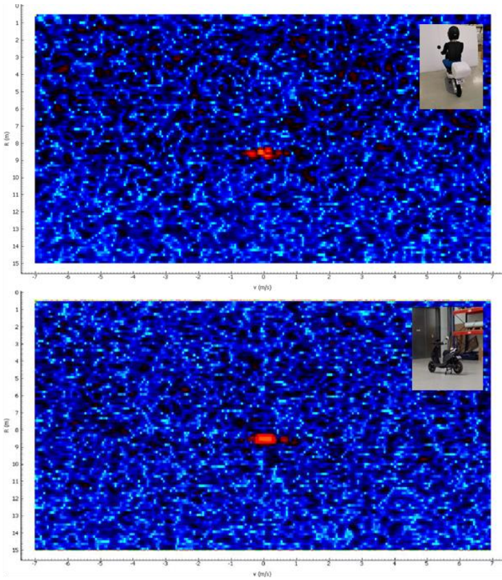
Figure A-33: Microdoppler response comparison 90 deg
