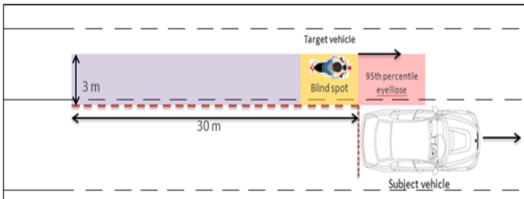
Figure 7: Must give blind spot warning to the driver
