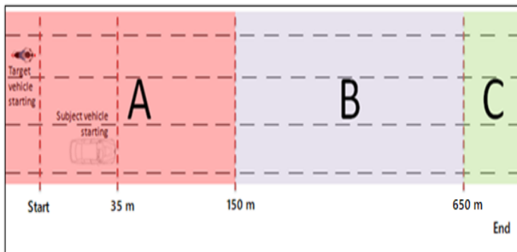
Figure 9: Test facility layout
