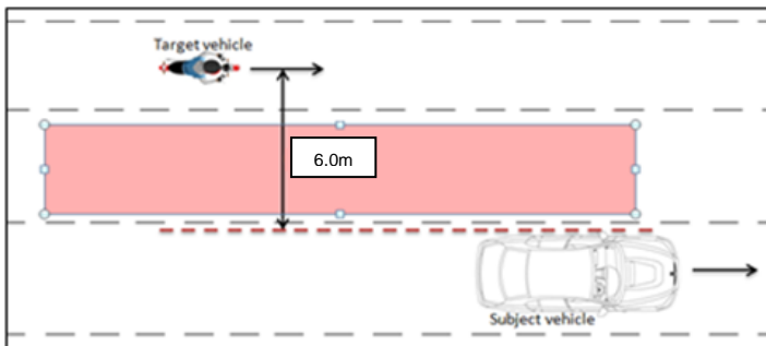
Figure 8: Target vehicle shall be maintained at 6.0 meters during test
