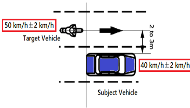
Figure 4: Target vehicle overtaking subject vehicle speed
