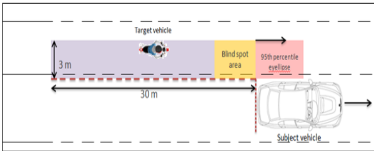
Figure 6: Might give blind spot warning to the driver
