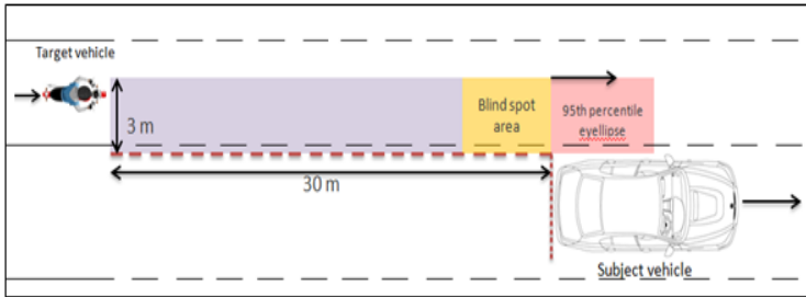
Figure 5: Must not give blind spot warning to the driver
