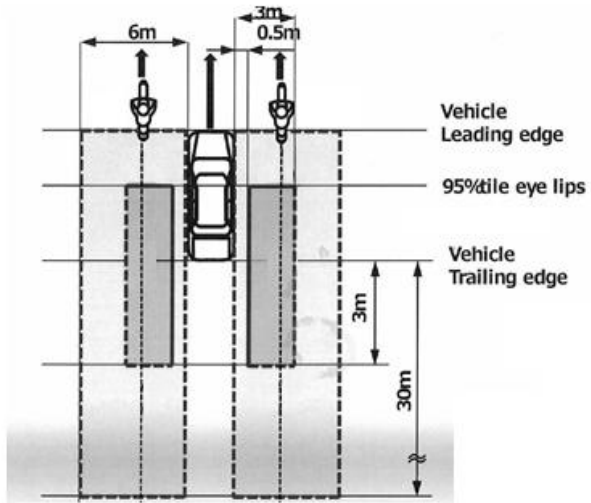
Figure A-5: Blind spot zone
