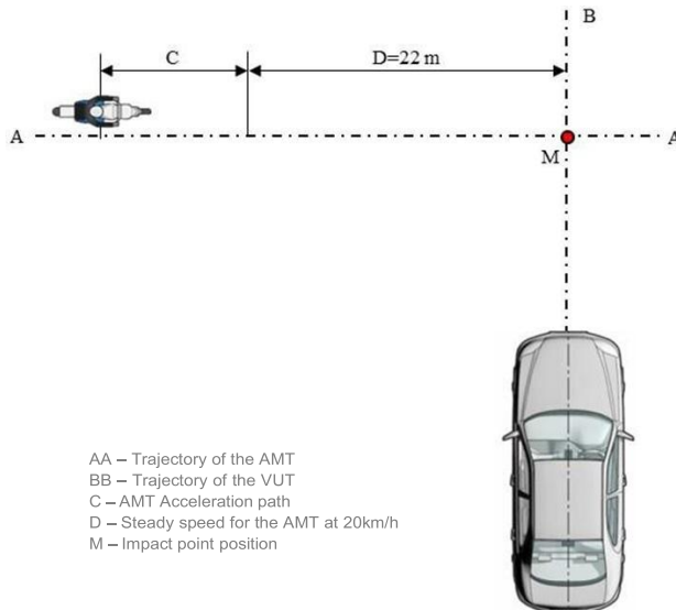
Figure 12: CMCrossing scenario (Motorcycle approaching from nearside)
