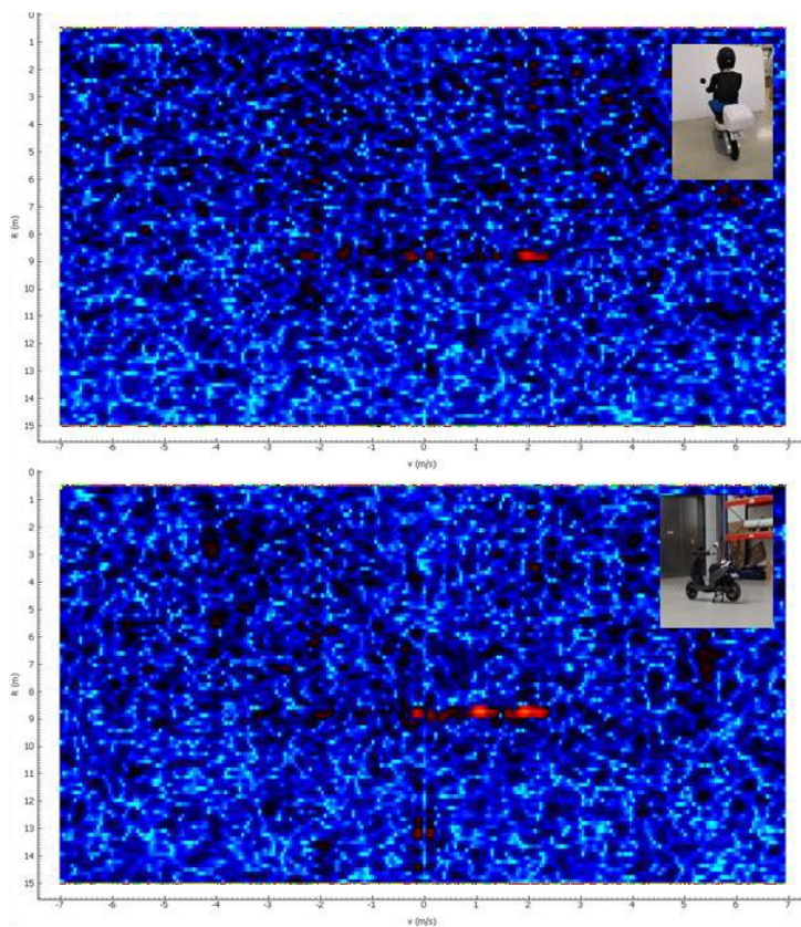
Figure A-34: MicroDoppler response comparison 45 deg
