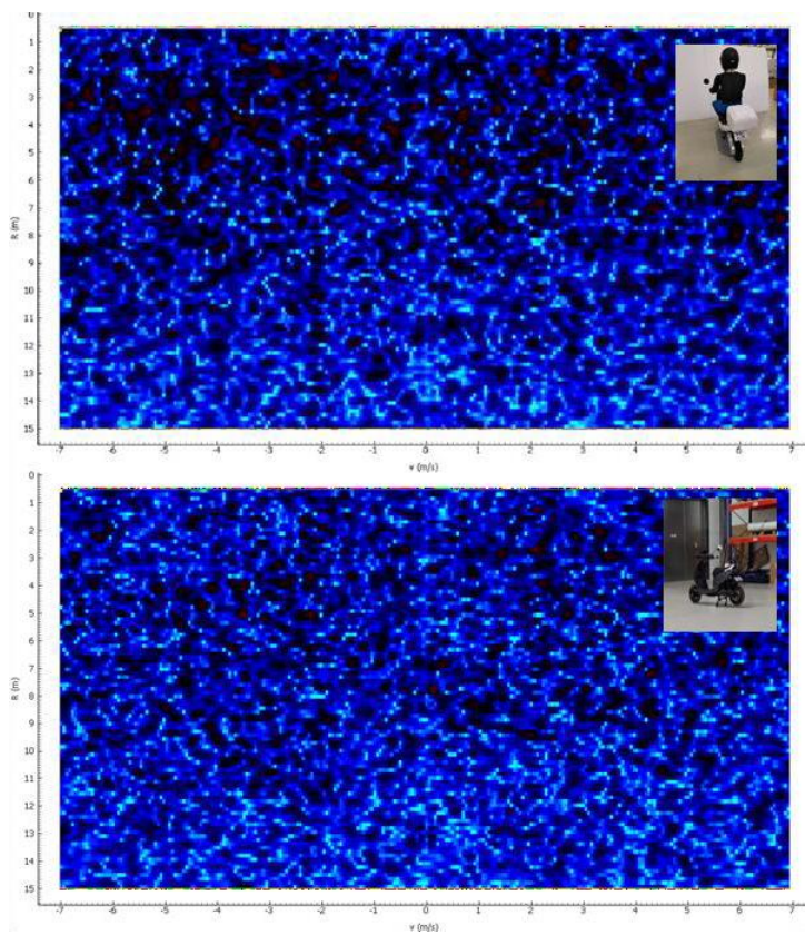
Figure A-35: MicroDoppler response comparison 0 deg
