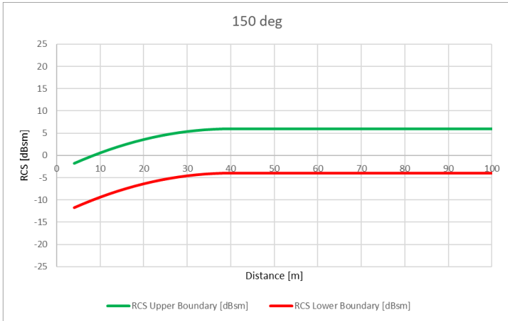
Figure A-11: Scooter Rider and Scooter Target RCS-Boundaries s (77GHz Sensor Bosch MRR-SGU) 150 deg
