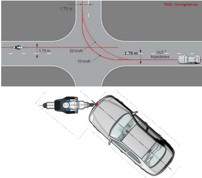
Figure 11: CMFtap scenario VUT and AMT paths
