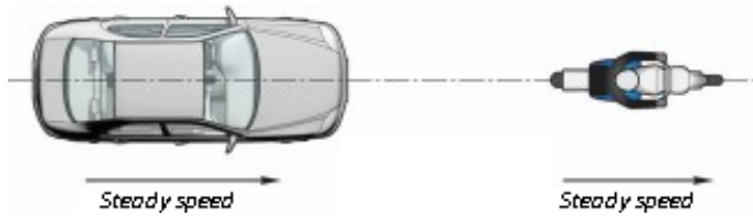
Figure 7: CMRm test scenario
