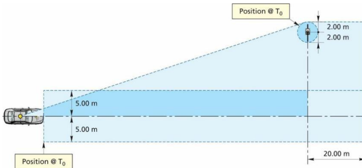
Figure 5: Free space requirements (nearside scenario only)
